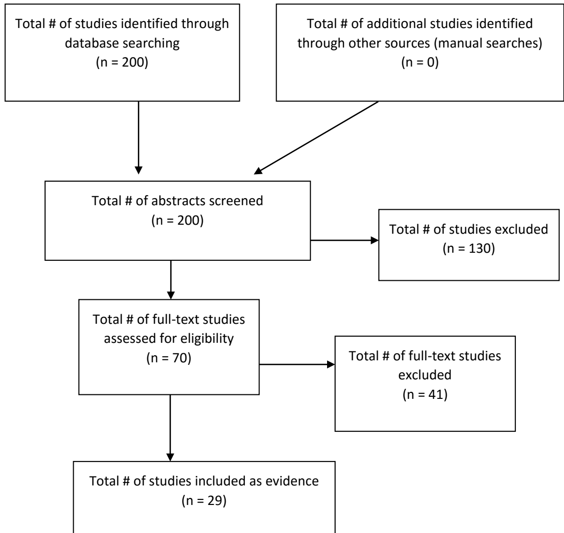
Figure 1 Article Flowchart
