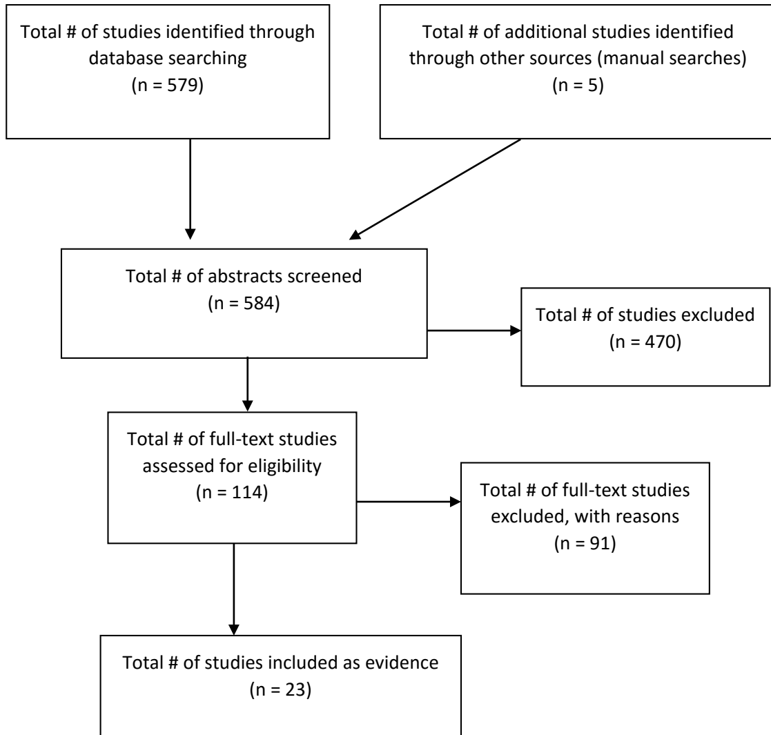
Figure 1. Article Flowchart
